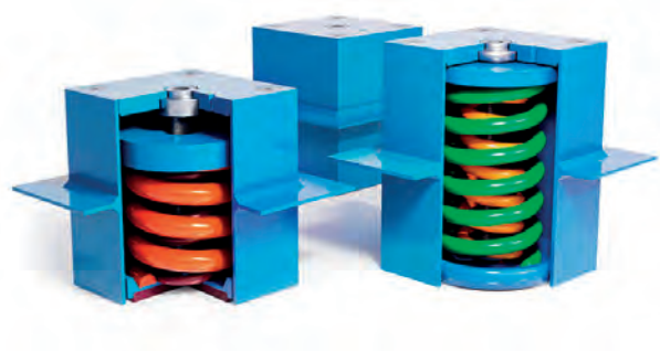
FZH2M-VSH + Sylomer ®
