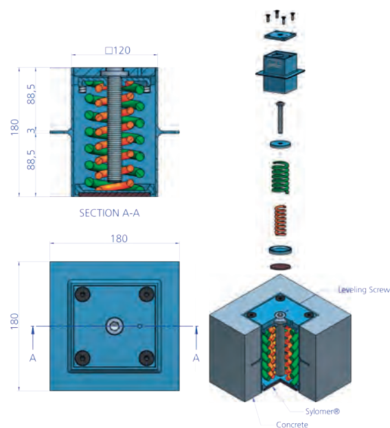
FZH2M-VSH + Sylomer ®
