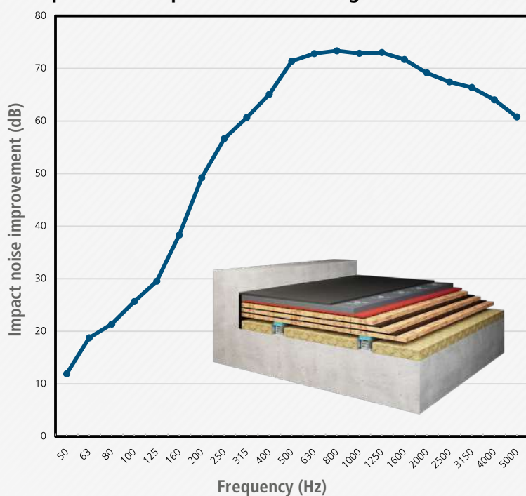
Impact noise improvement according to EN ISO 10140-3
